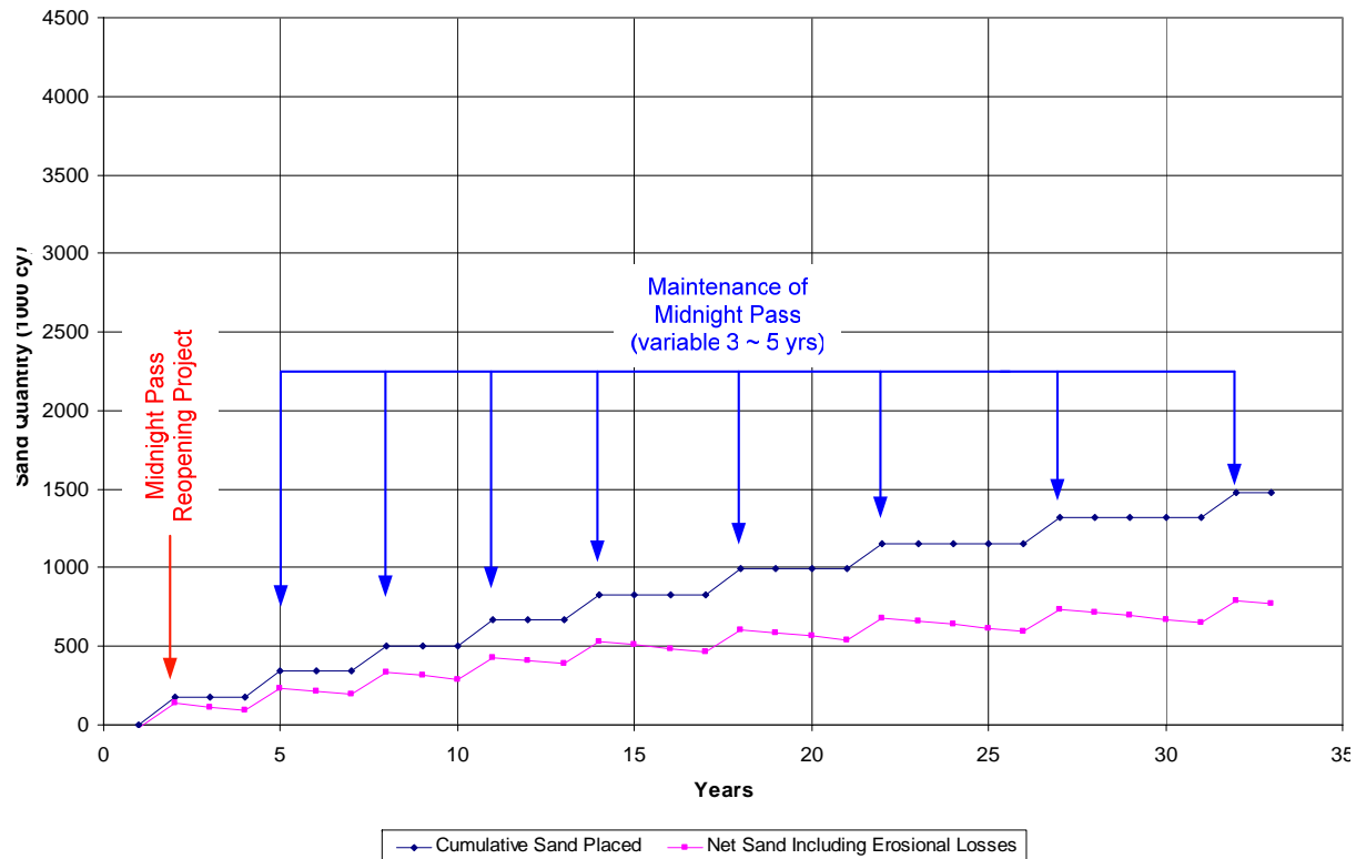
Figure 33(a)-10 Casey Key Sediment Budget based upon 35:65 Sand Allocation Plan
