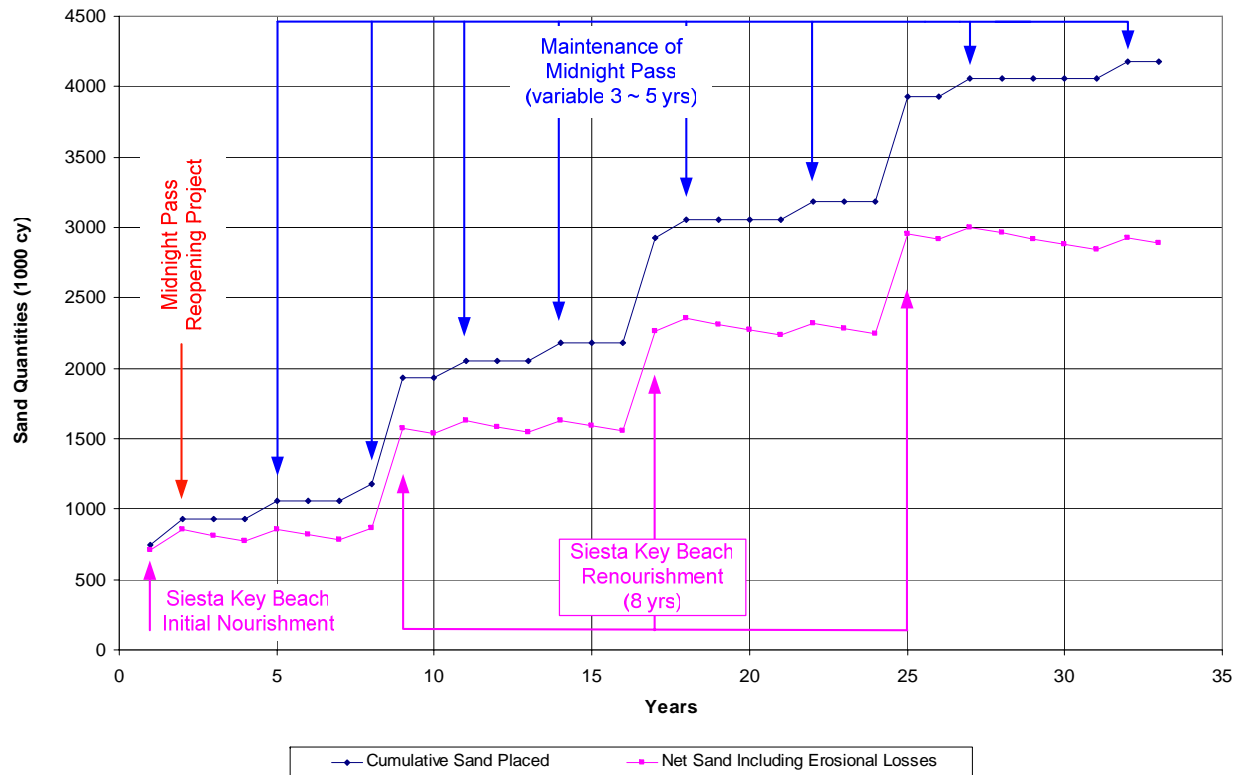
Figure 33(a)-9 Siesta Key Sediment Budget based upon 35:65 Sand Allocation Plan
