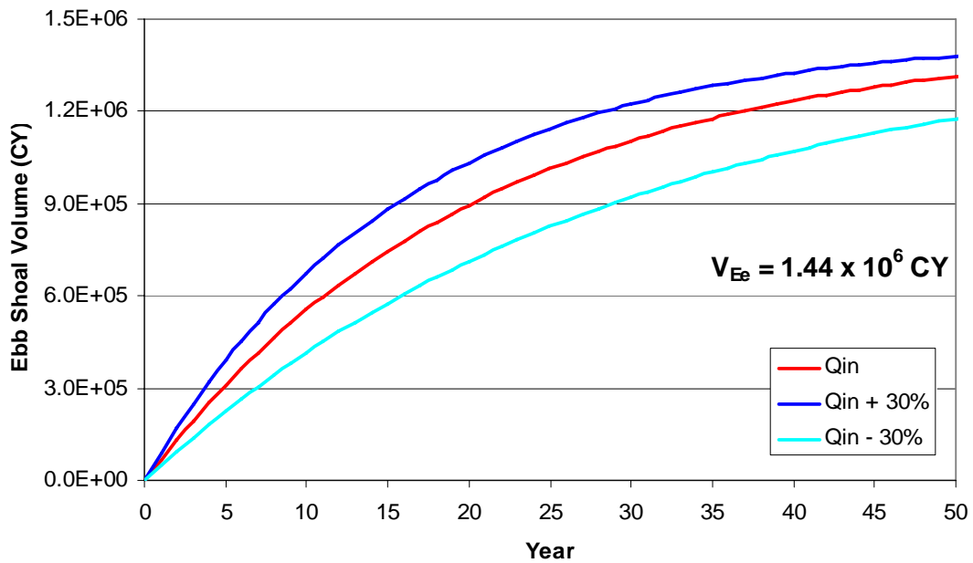
Figure 33(a)-1 Volume Growth of Ebb Shoal at Midnight Pass Following Pass Reopening
